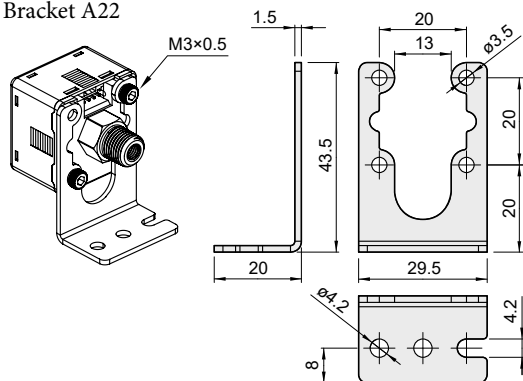
Bracket A22
