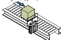
Using as stopper cylinder
