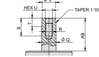
Piston rod end detail for double-sided arm:
