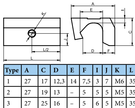
Bracket
