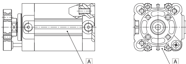
A Sensor must be placed in the groove closest to the telescopic magnetic shaft
